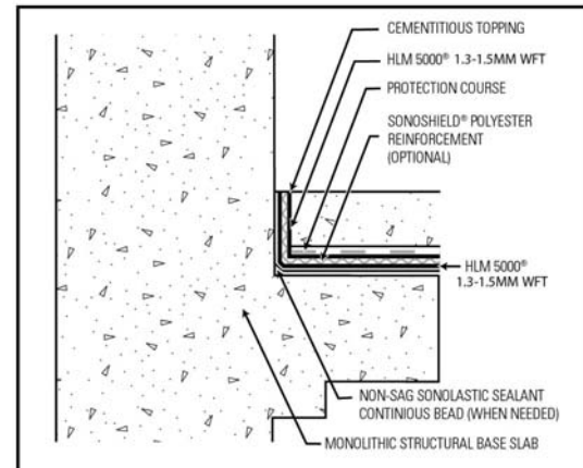
Inside Corner Detail (Static)
